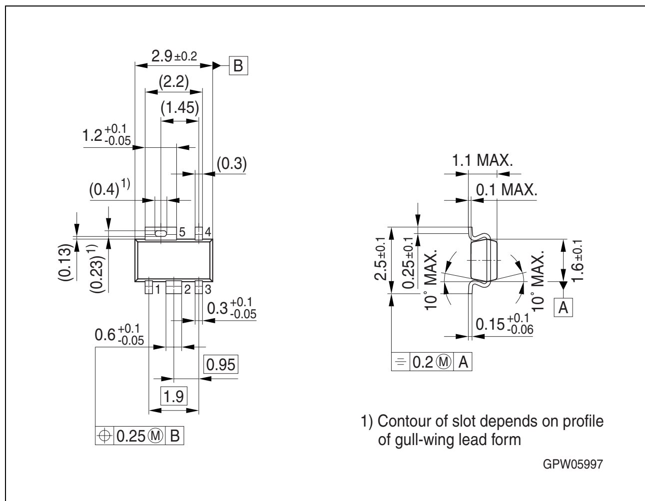
Figure 4 Outline PG-SCT595-5
