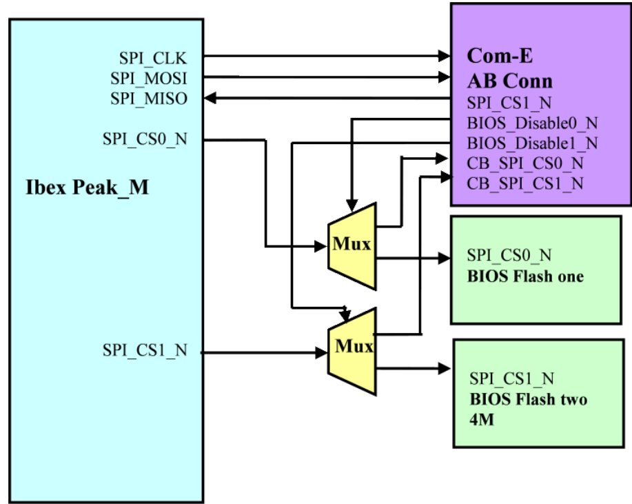
Figure 4-11 SPI Interface Diagram
