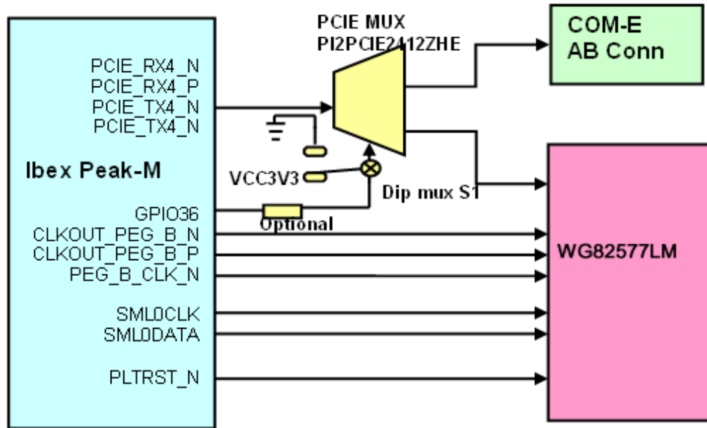
Figure 4-10 WG82577LM Connection Diagram
