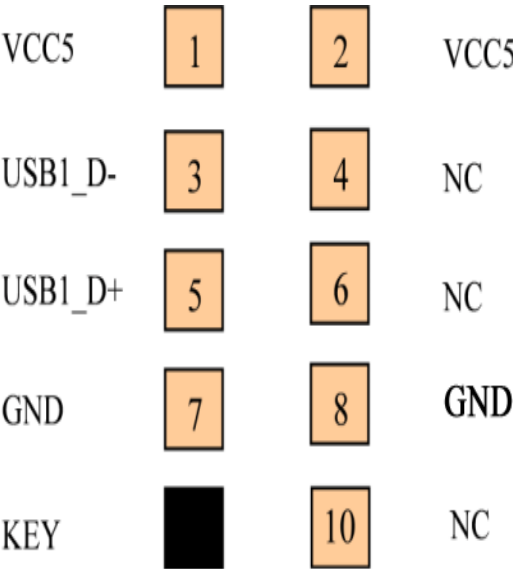
Figure 3-3 eUSB Flash Header Pin Definition
