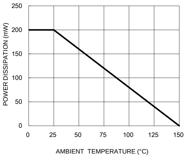
Fig.7 Power Dissipation
