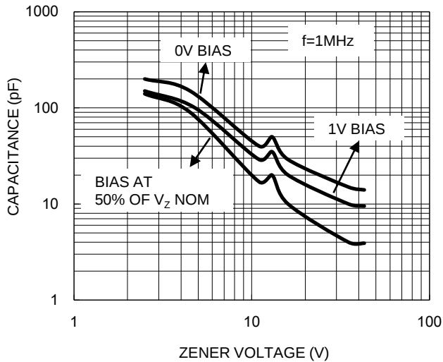
Fig.5 Typical Capacitance
