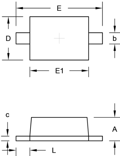
SOD-323F
