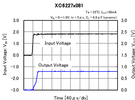
(9) Input Transient Response
