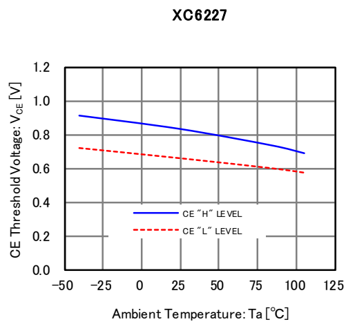
(6) CE Pin Threshold Voltage vs. Ambient Temperature
