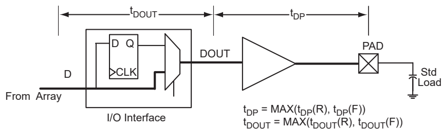
FIGURE 2-5: OUTPUT BUFFER MODEL AND DELAYS (EXAMPLE)
