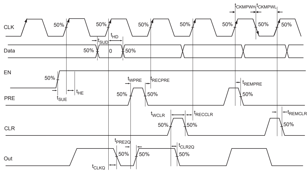
FIGURE 2-24: TIMING MODEL AND WAVEFORMS
