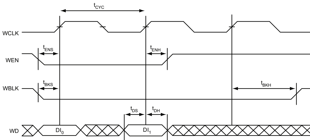
FIGURE 2-35: FIFO WRITE
