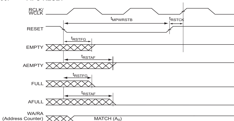
FIGURE 2-36: FIFO RESET
