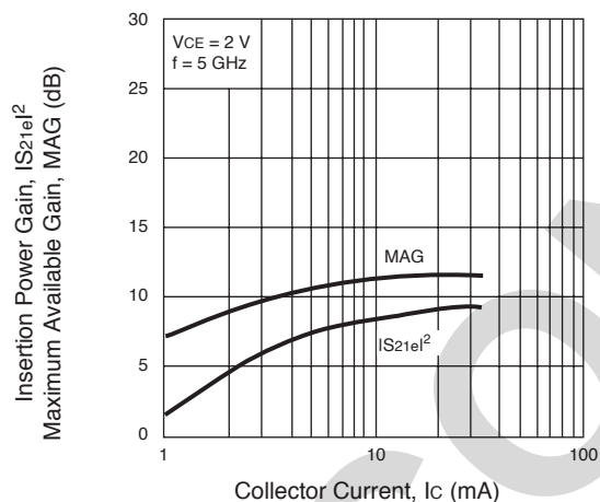
MAXIMUM AVAILABLE GAIN, INSERTION POWER GAIN vs. COLLECTOR CURRENT
