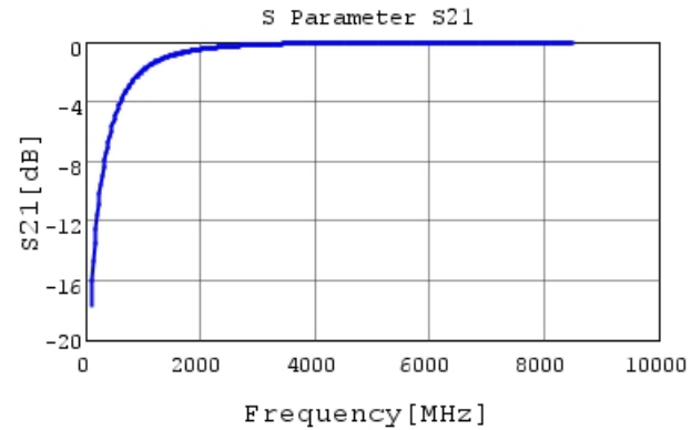
GCQ1555C1H2R1WB01 S21 DCOV, 25degC
