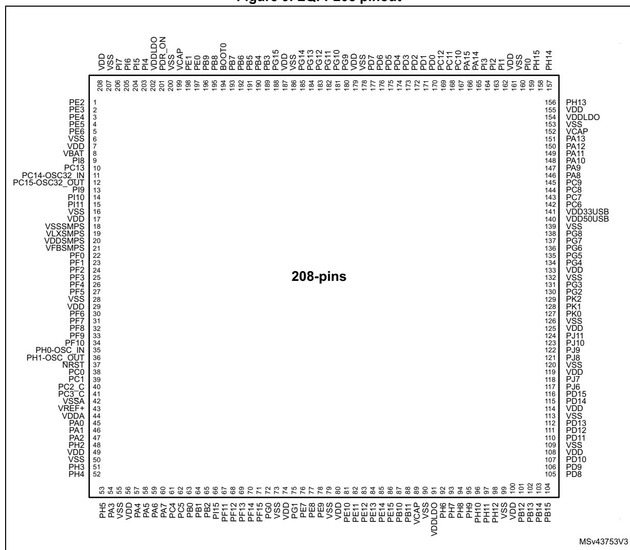
Figure 9. LQFP208 pinout
