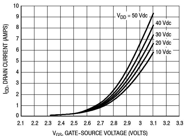
Figure 5. Drain Current versus Gate-Source Voltage
