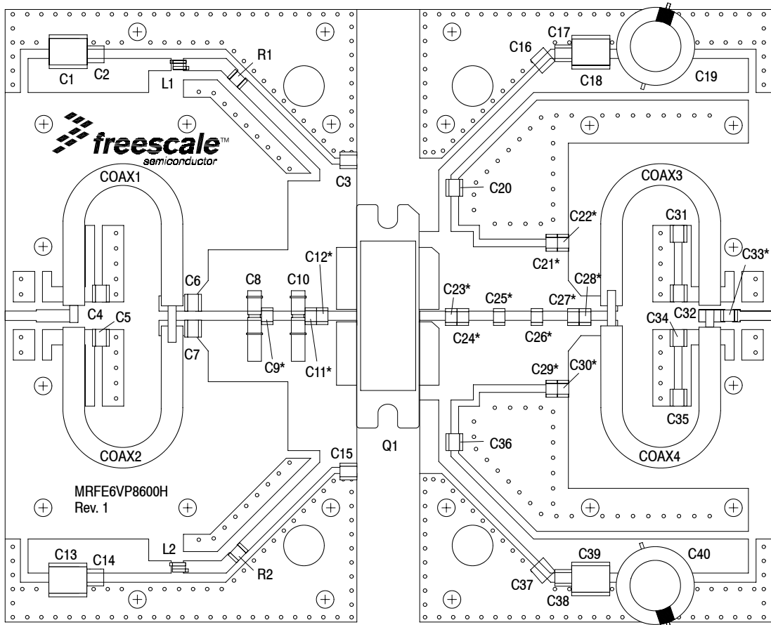
Figure 14. MRFE6VP8600HR6(HSR6) Broadband Test Circuit Component Layout — 470-860 MHz
