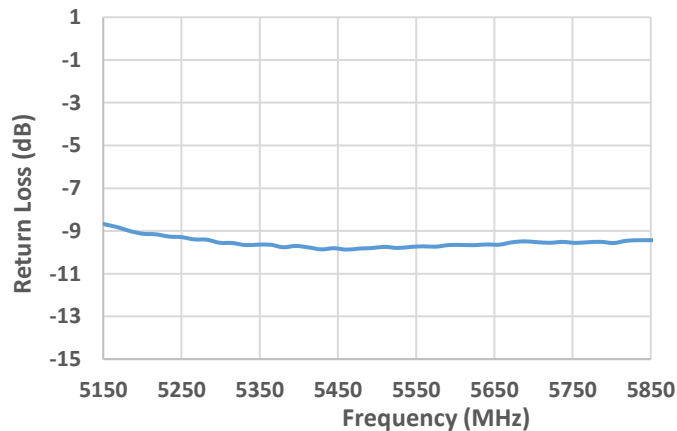
Return Loss (5150 – 5850 MHz)
