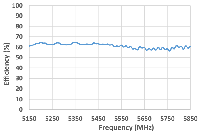
Efficiency (5150 – 5850 MHz)
