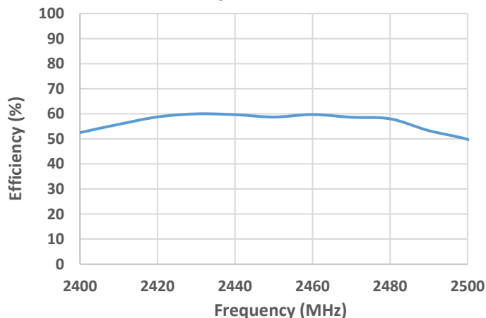
Efficiency (2400 – 2500 MHz)
