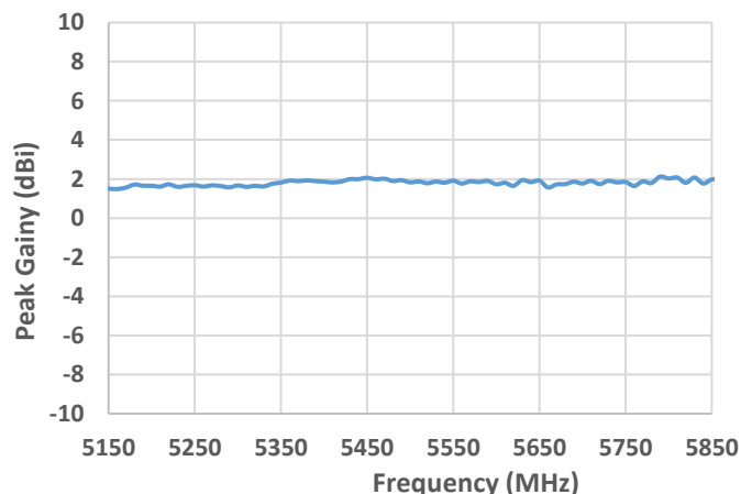
Peak Gain (5150 – 5850 MHz)
