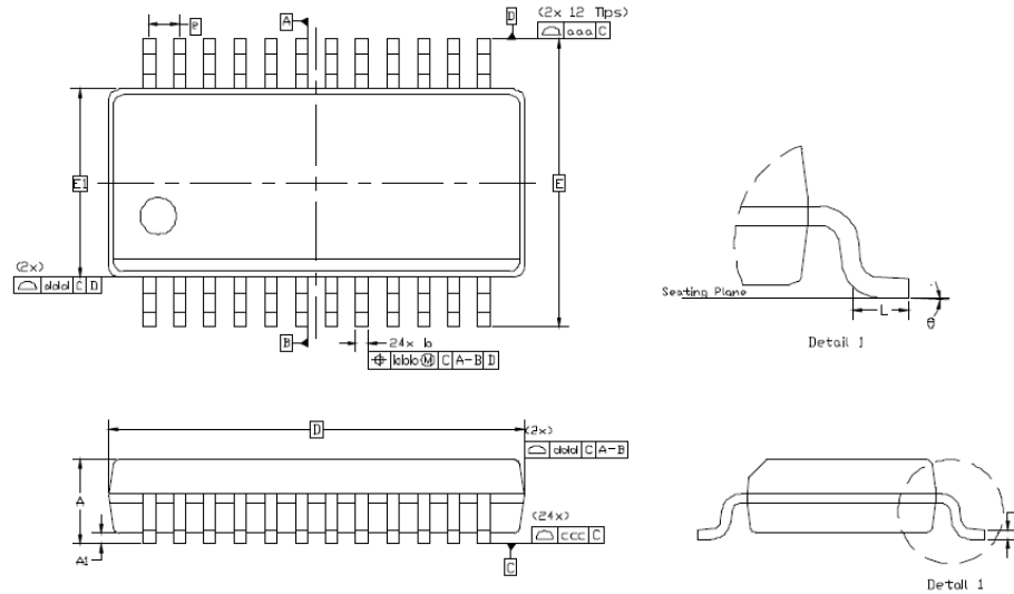
Figure 6. 24-Pin SSOP
