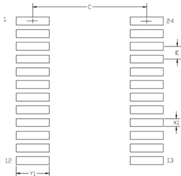
Figure 7. PCB Land Pattern
