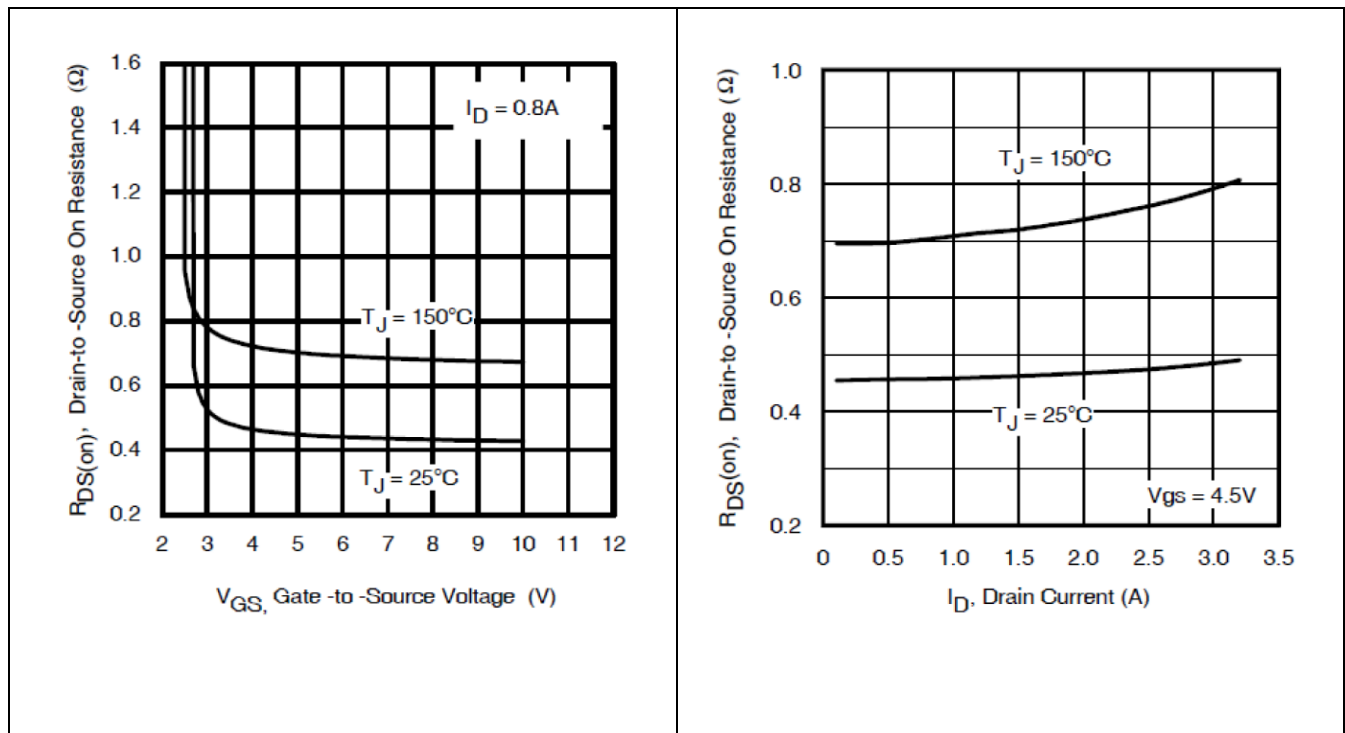
Figure 6 Typical On-Resistance Vs. Gate Voltage
