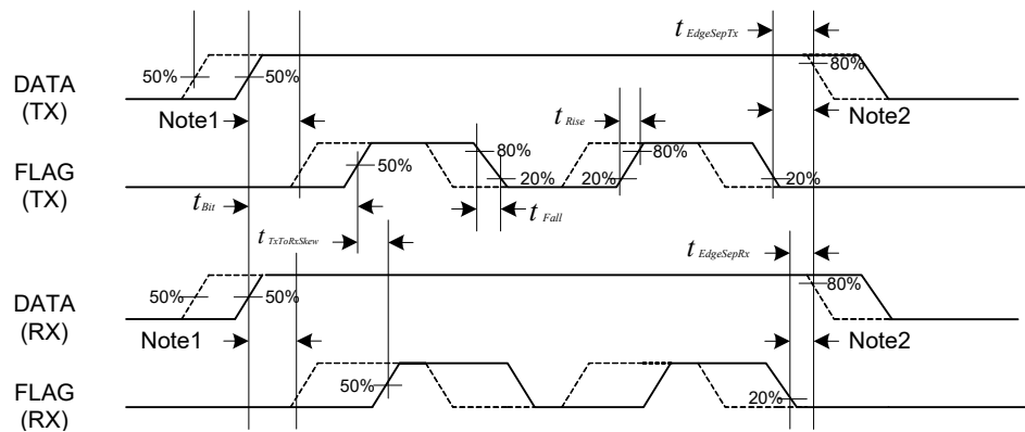
Figure 78. DATA and FLAG Signal Timing
