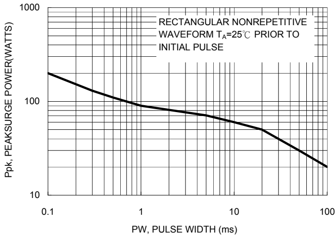
FIG. 2- MAXIMUM SURGE POWER
