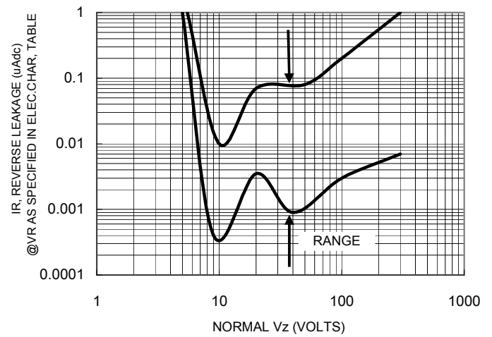
FIG. 3- TYPICAL REVERSE LEAKAGE
