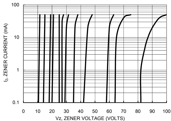
FIG. 7- V_z = 11 THRU 91 VOLTS
