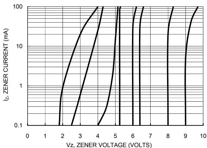
FIG. 6- V_z = 6.8 THRU 10 VOLTS
