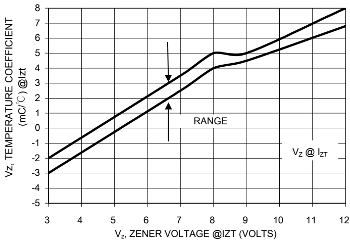
FIG.4- UNIT 6.8 TO 12 VOLTS
