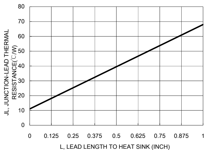
FIG. 9- TYPICAL THERMAL RESISTANCE
