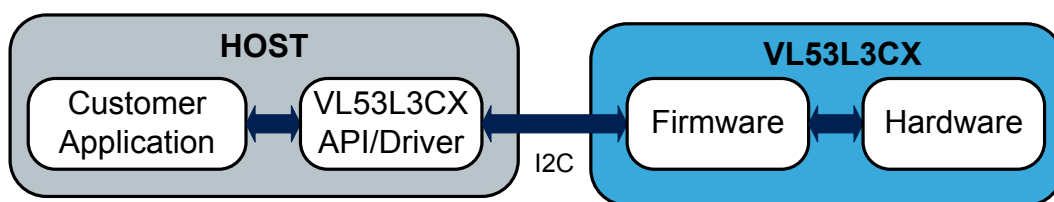
Figure 4. VL53L3CX system functional description
