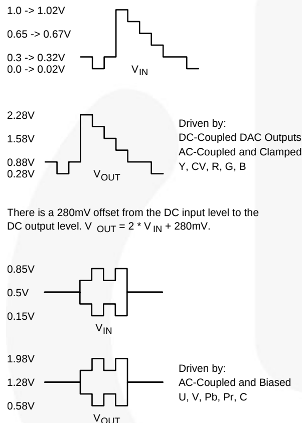
Figure 12. Typical Voltage Levels
