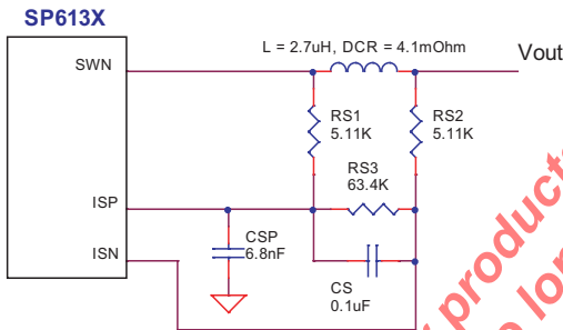
Figure 2- Over-current detection circuit for I_{MAX} > 60\text{mV} / \text{DCR}
