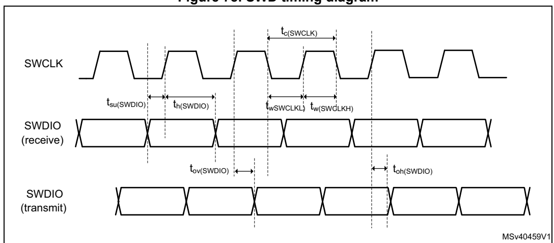
Figure 78. SWD timing diagram
