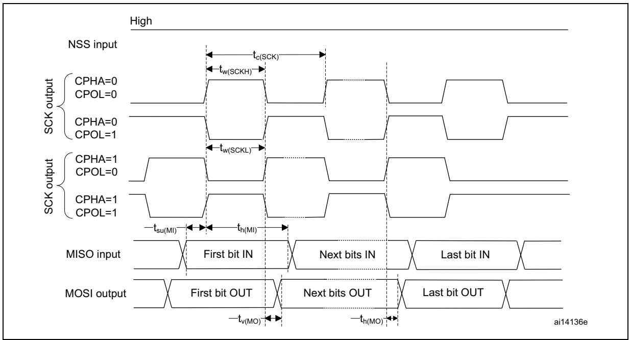
Figure 65. SPI timing diagram - master mode
