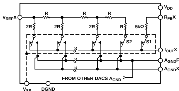
DIGITAL INTERFACE CONNECTIONS OMITTED FOR CLARITY. SWITCHES S1 AND S2 ARE CLOSED, AND V_{\text{DD}} MUST BE POWERED.
