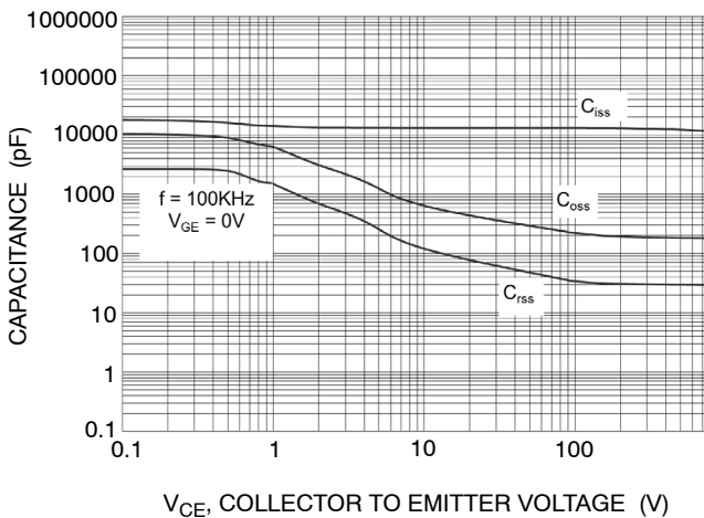
Figure 27. Capacitance Charge
