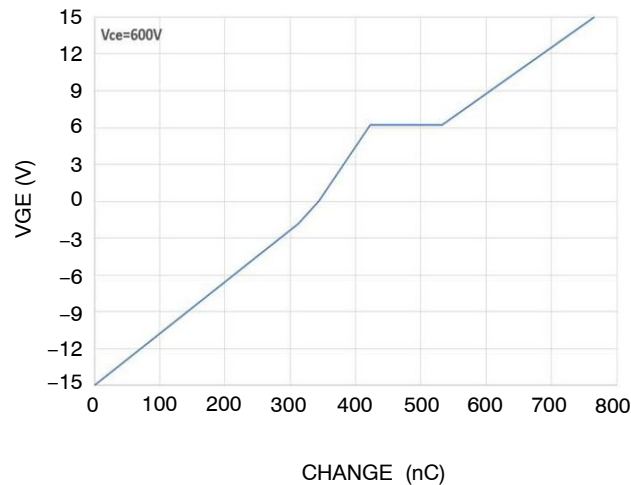
Figure 28. Gate Voltage vs. Gate Charge
