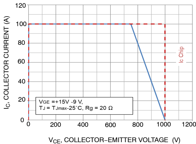
Figure 26. RBSOA
