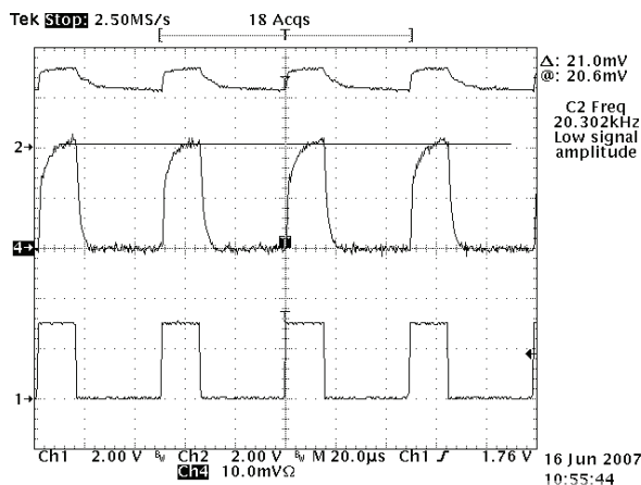
PWM Minimum on time 15 \mu S 20kHz CH1: PWM Signal CH2: Anode of LED CH4: LED current 10mA/div
