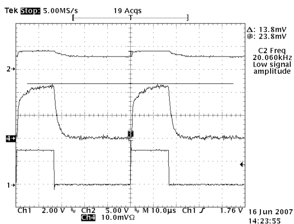
PWM Minimum on time 15μS Single LED 20kHz
