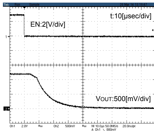
Figure.49 Turn off response 7 (BUS1DJC3GWZ V_{IN} =1.2V)
