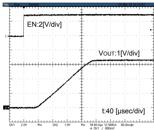
Figure.56 Turn on response 11 (BUS1DJC3GWZ VIN=3.3V)
