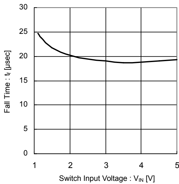
Figure 47. Fall Time vs Switch Input Voltage (BUS1DJC3GWZ)
