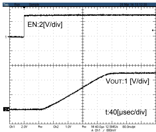
Figure.54 Turn on response 10 (BUS1DJC3GWZ VIN=2.5V)
