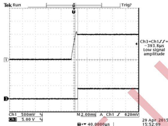
Figure 8. Typical Start-up Using Remote ON/OFF ( V_{in}=12.0V , V_o=1.0V , I_o=0A )
