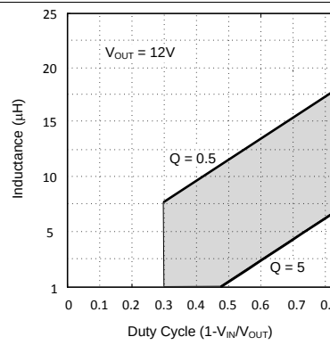
Figure 18. Minimum Inductance Requirements for (b) f_s = 1.25 MHz
