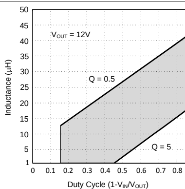
Figure 17. Minimum Inductance Requirements for (a) f_s = 600 kHz
