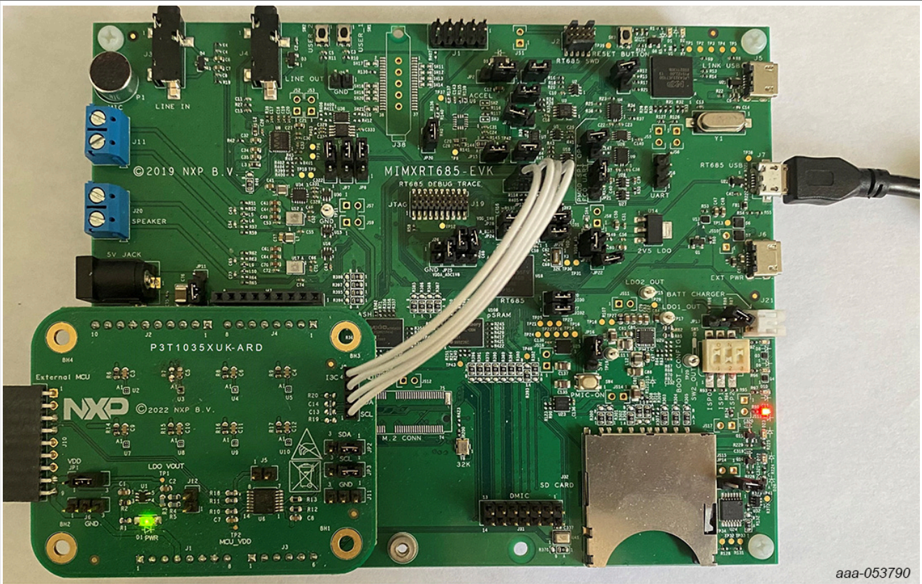
Use J7 (USB Micro-B connector) on MIMXRT685-EVK for power supply and GUI communication port. Figure 3. P3T1035XUK-ARD evaluation board connecting to the MIMXRT685-EVK MCU board
