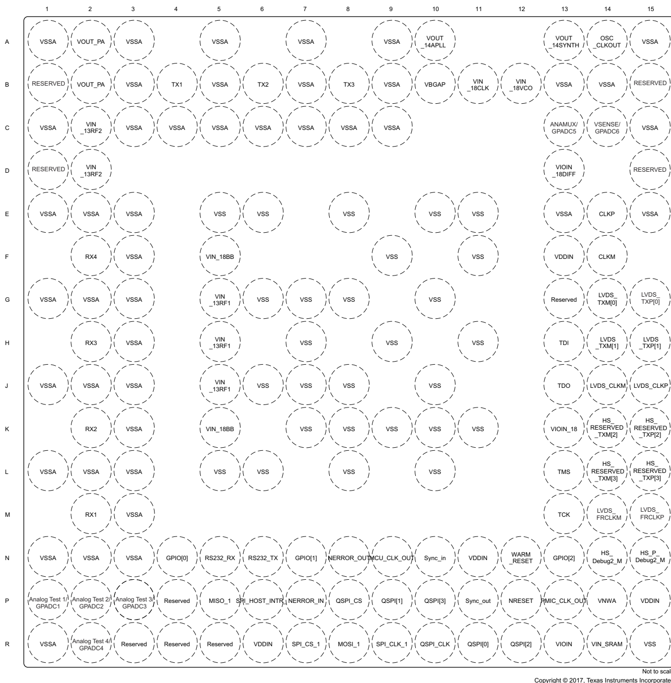
Figure 7-1. Pin Diagram
