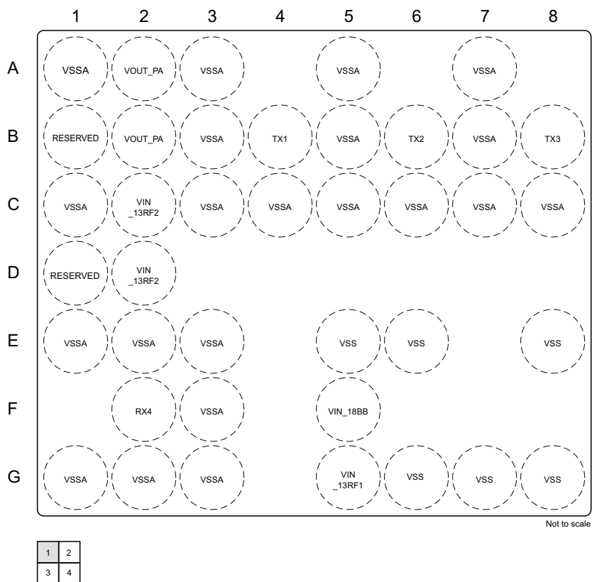
Figure 7-2. Top Left Quadrant
