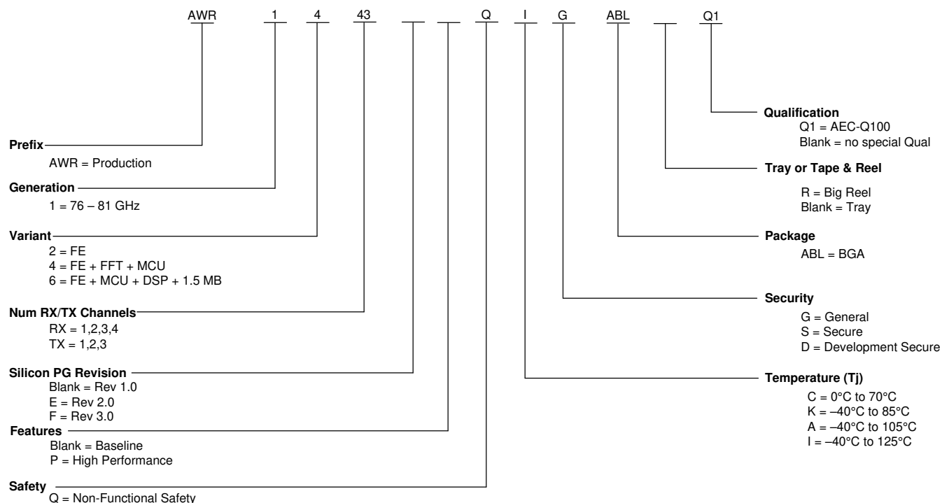
Figure 11-1. Device Nomenclature
