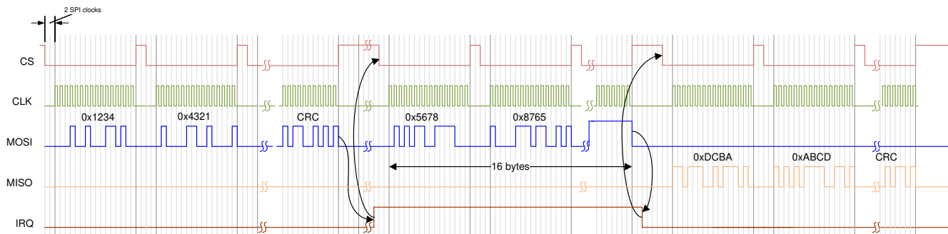
Figure 8-11. SPI Communication
