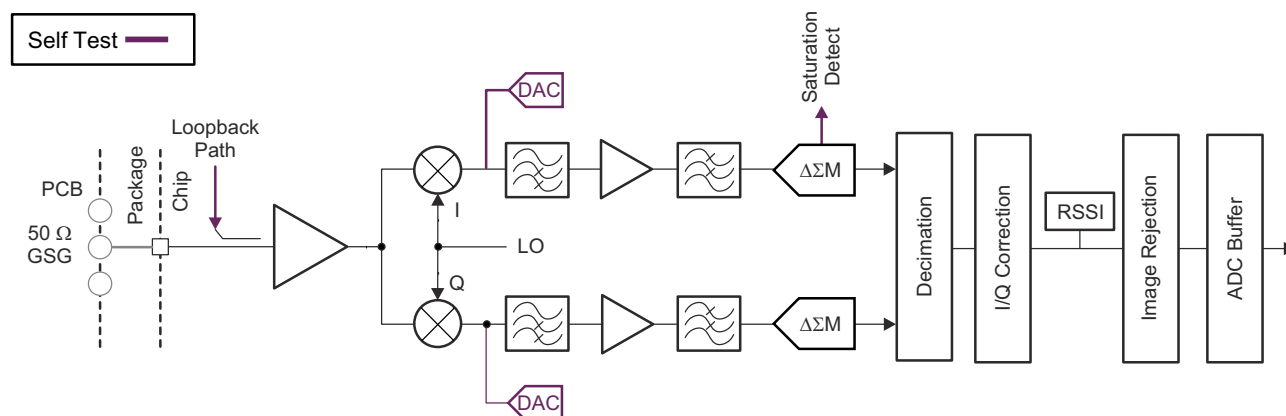
Figure 9-5. Receive Subsystem (Per Channel)
