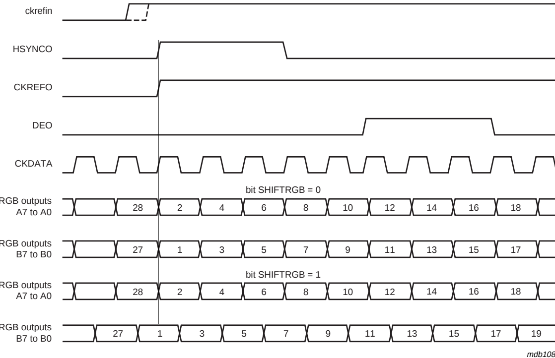
HSYNCO, DEO, CKREFO and RGB outputs A7 to A0 are referred to the rising edge of ckrefin. CKREFO is LOW during 8 clock pulses.
