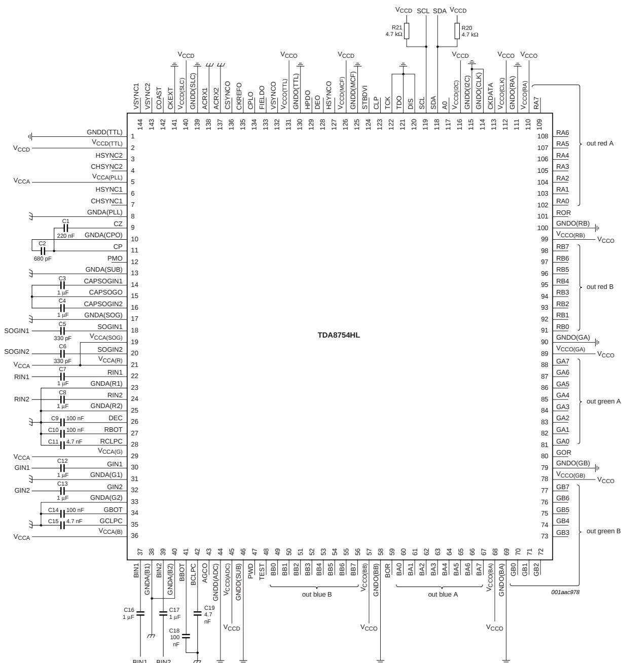
Fig 10. Application diagram
