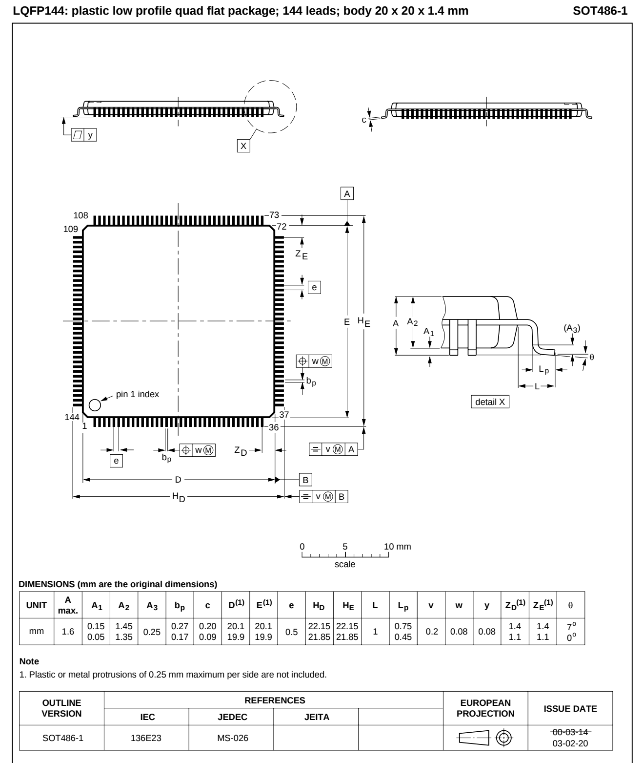
Fig 11. Package outline SOT486-1 (LQFP144)
