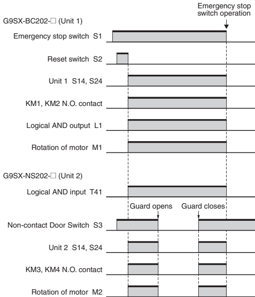
Timing chart
