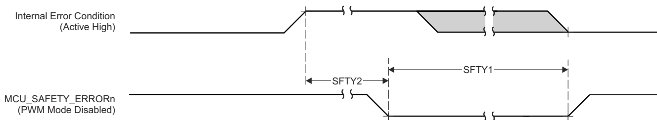
Figure 6-10. MCU_SAFETY_ERRORn Switching Characteristics
