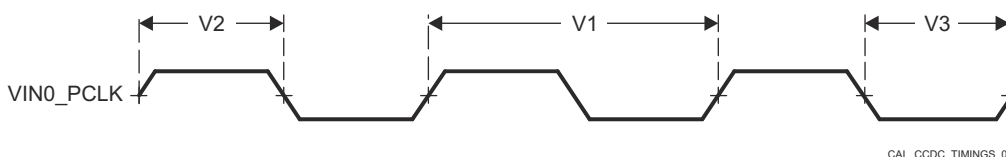
Figure 6-30. LVDSRX Input Clock Signal
