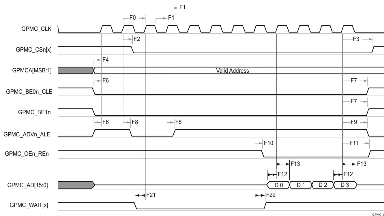
Figure 6-49. GPMC and NOR Flash—Synchronous Burst Read—4x16-bit (GpmcCLKDivider = 0)
