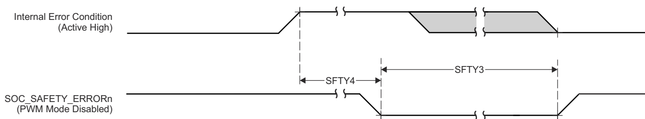
Figure 6-11. SOC_SAFETY_ERRORn Switching Characteristics
