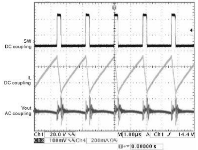
14. Steady-State Waveform
