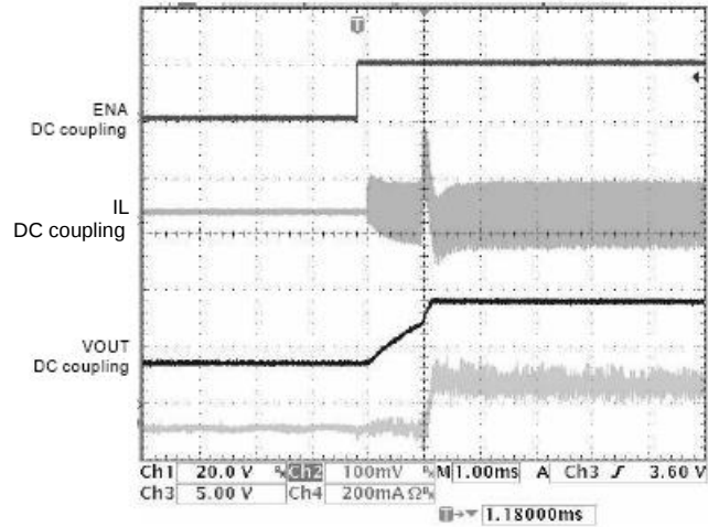
13. Startup Waveform
