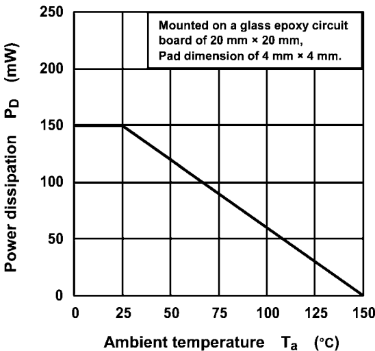
Fig. 8.4 P_D - T_a
