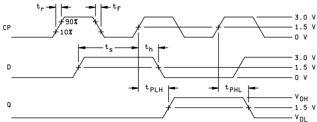
PROPAGATION DELAY TIMES
