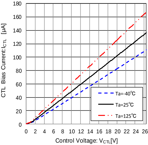
Figure 55. CTL Current vs CTL Voltage
