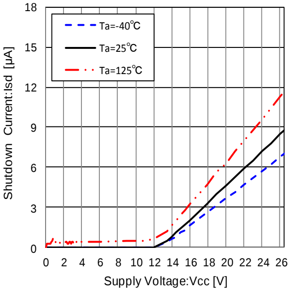
Figure 47. Shutdown Current ( V_{\text{CTL}}=0\text{V} )
