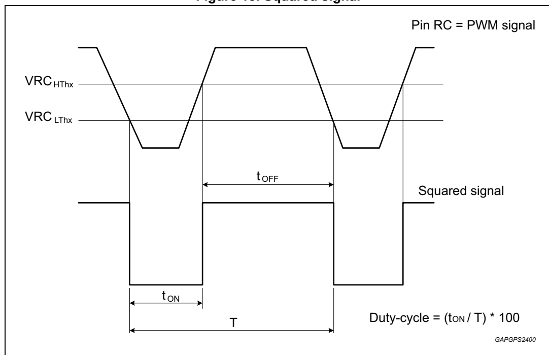
Figure 18. Squared signal
