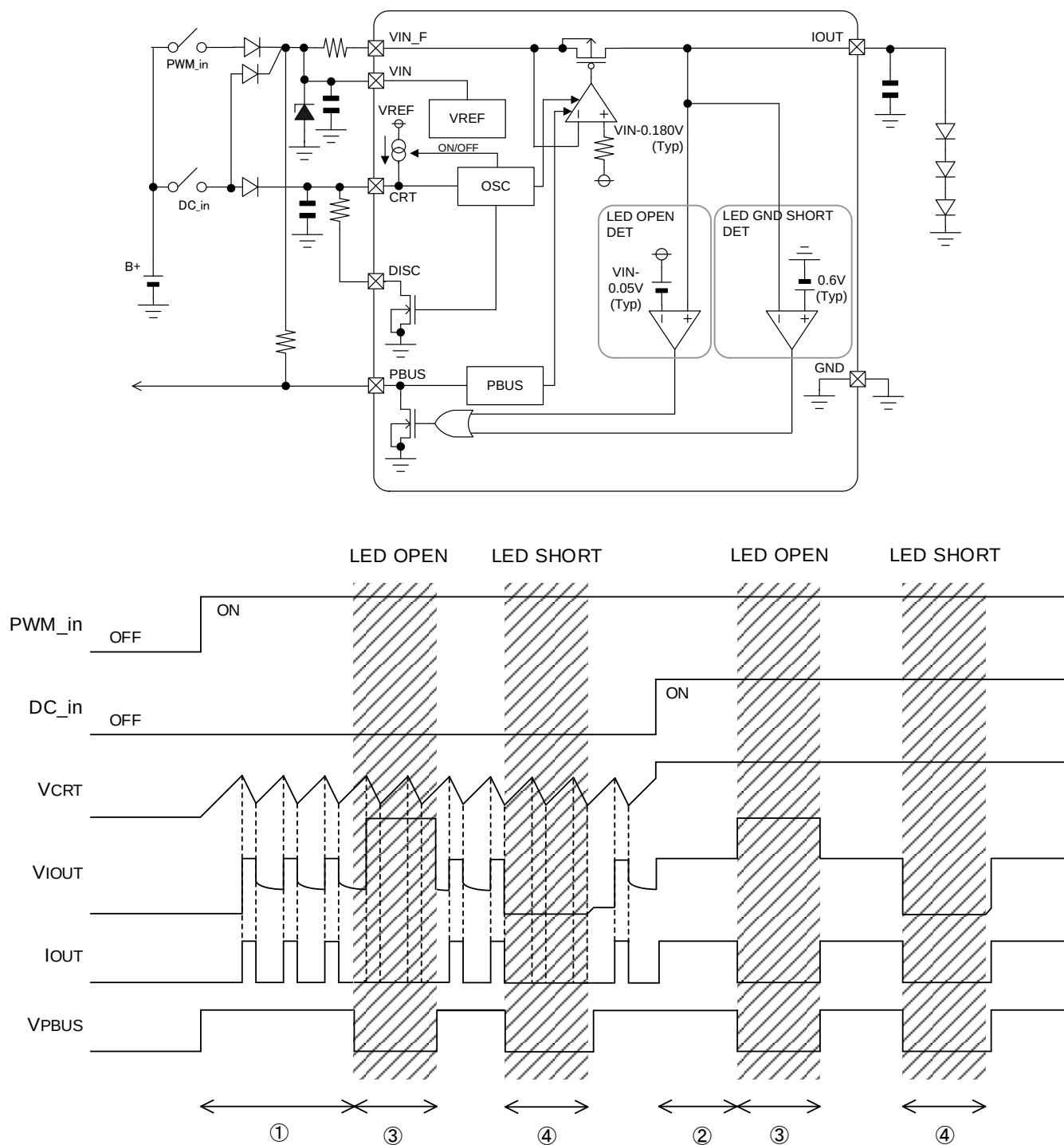
Figure 24. Timing Chart
