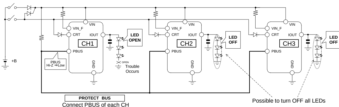
Figure 21. PBUS Function
