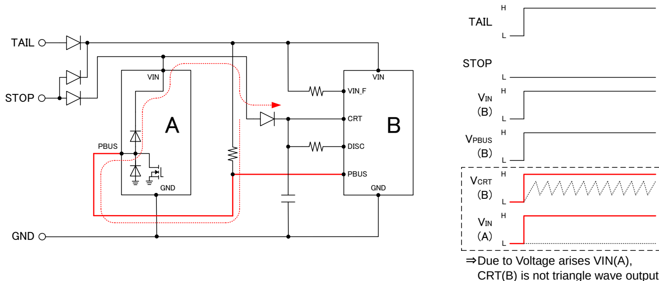
Figure 23. Application Example
