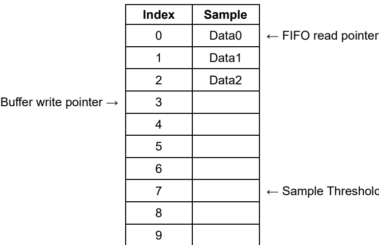
Figure 2. Buffer Filling
