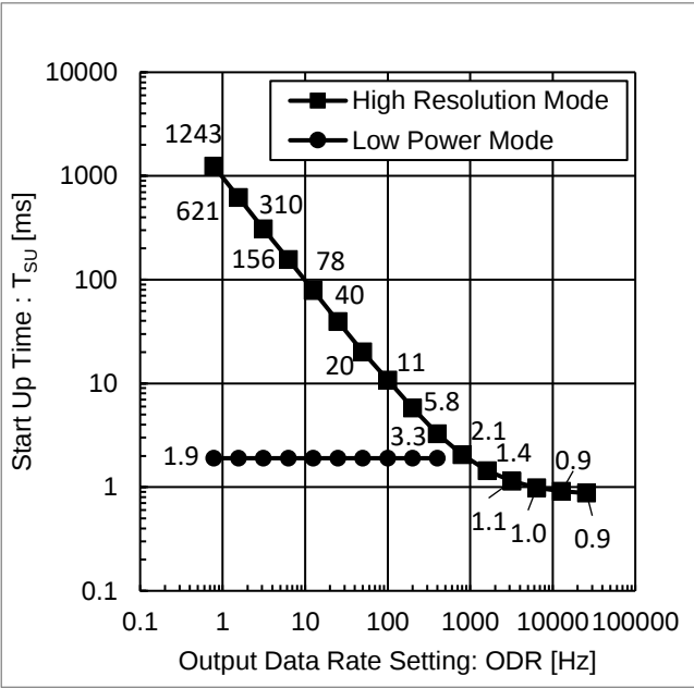
Figure 11. Start Up Time vs ODR
