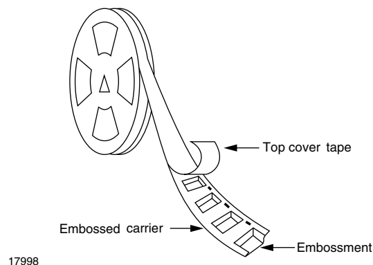
Fig. 24 - Tape and Reel Shipping Medium
