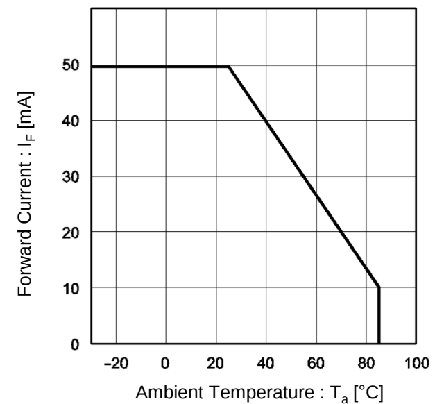
Fig.3 Forward Current Falloff
