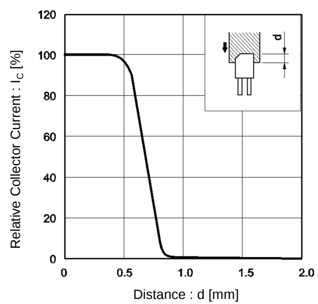
Fig.2 Relative Output Current vs.Distance (II)
