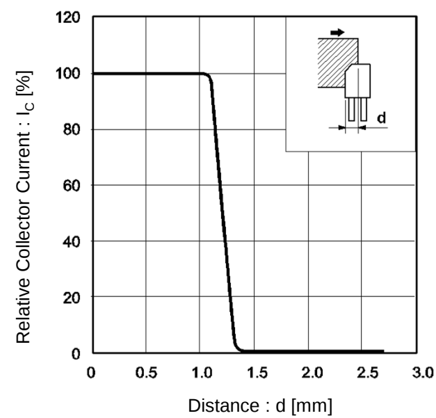
Fig.1 Relative Output Current vs.Distance (I)
