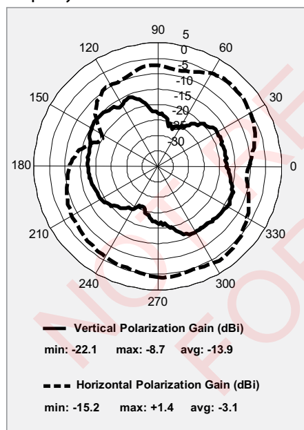
Frequency = 2480 MHz
