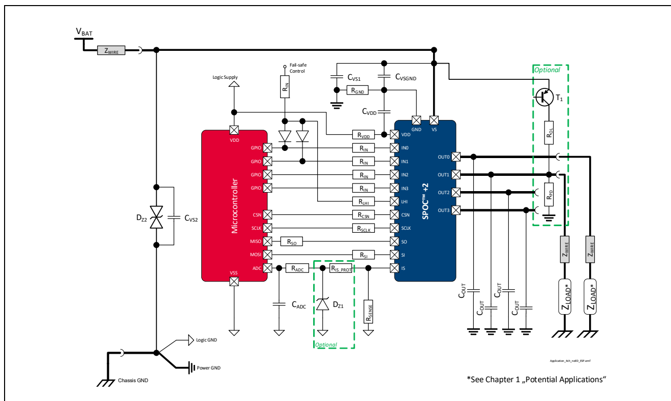
Figure 46 Application Diagram
