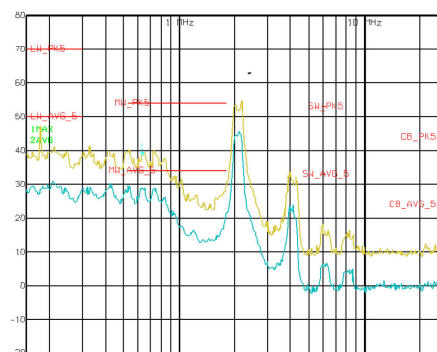
CISPR 25 EMI Performance - 150kHz to 30MHz
