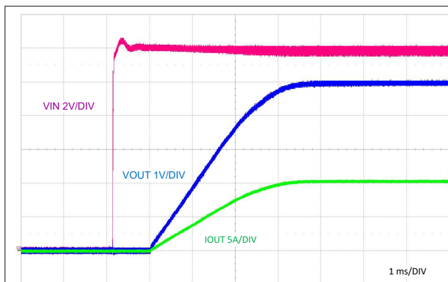
Figure 8-35. Start-Up Characteristic
