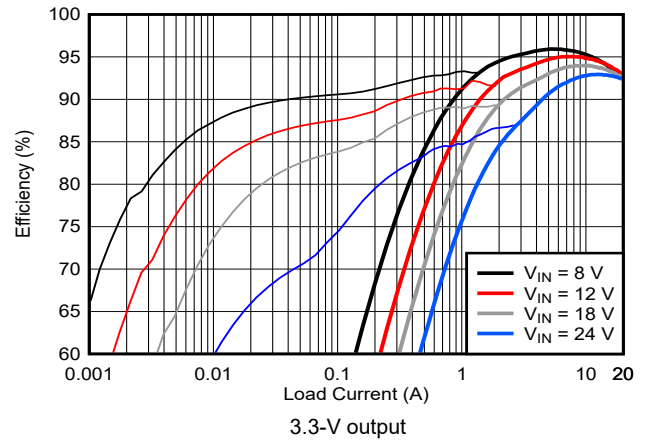
Figure 8-41. Efficiency vs I_{OUT} , Log Scale
