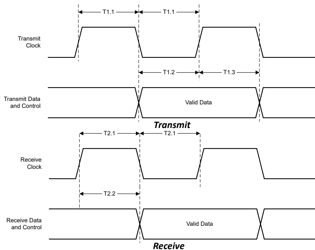
Figure 7-1. MII Timing
