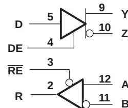
SN65MLVD203, SN65MLVD207
