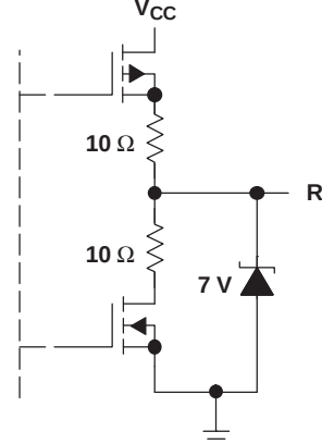
RECEIVER OUTPUT
