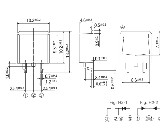
H2 Package: SC-83 similar
