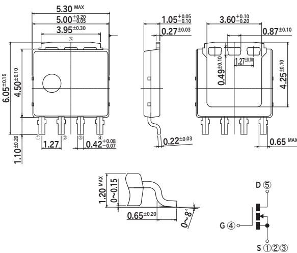
G7 Package: MO-235B similar
