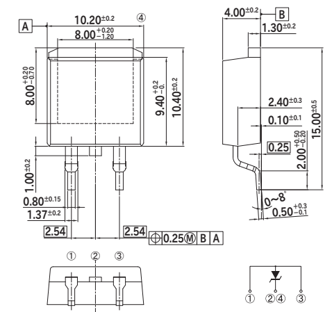
H6 Package: TO-263AB
