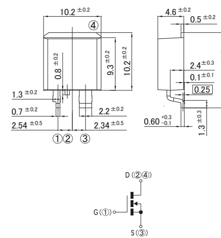
H5 Package: SC-83 similar
