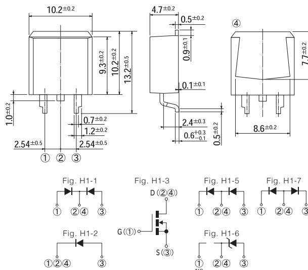
H1 Package: SC-83 similar
