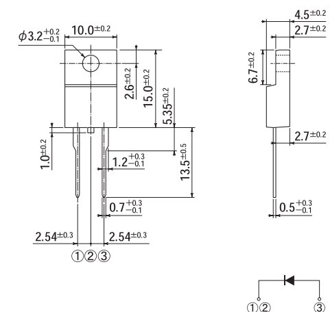
J1 Package: SC-91A
