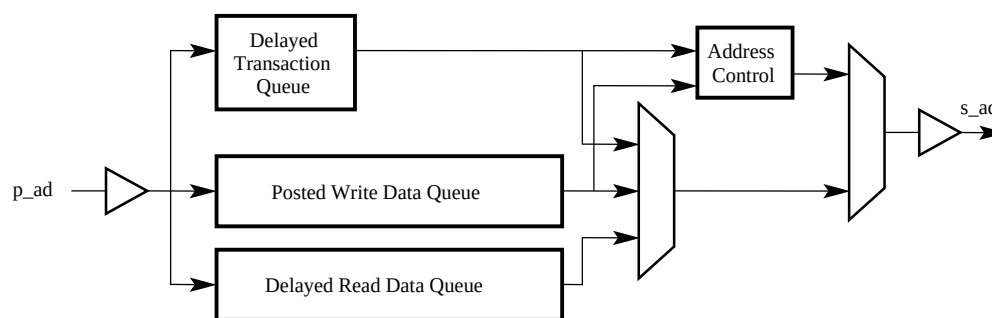
Figure 4. 21152 Downstream Data Path
