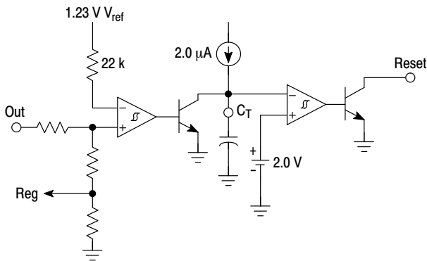
Figure 18. Reset Circuit
