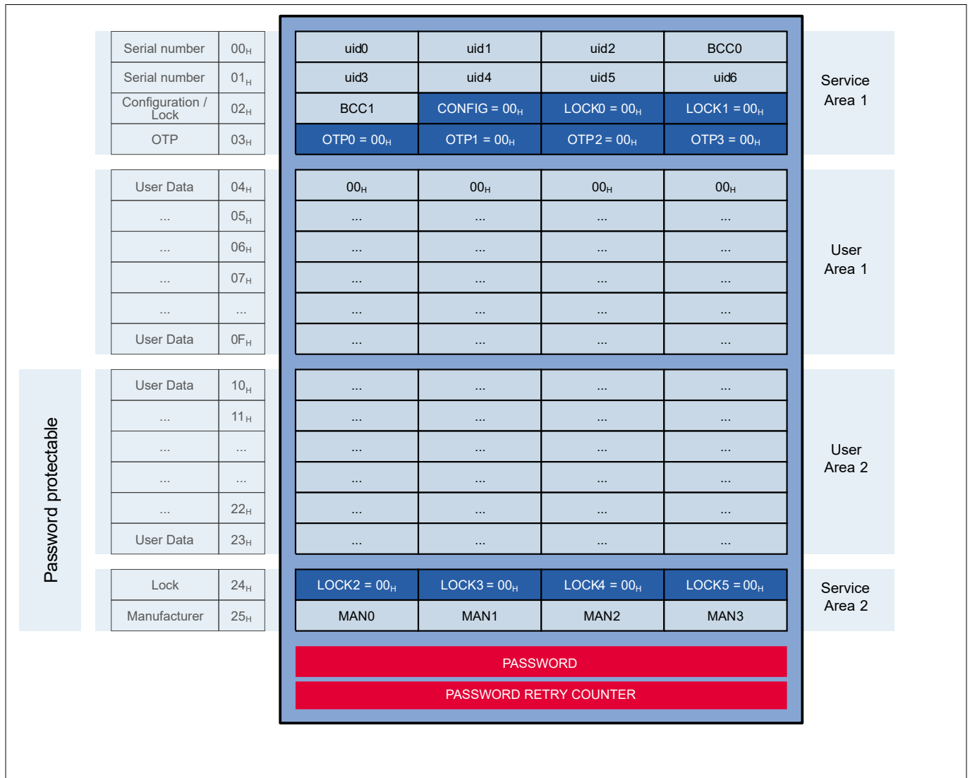
Figure 17 my-d™ move transport configuration
