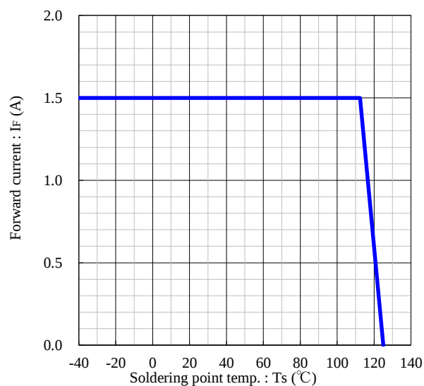
Maximum ratings of forward current
