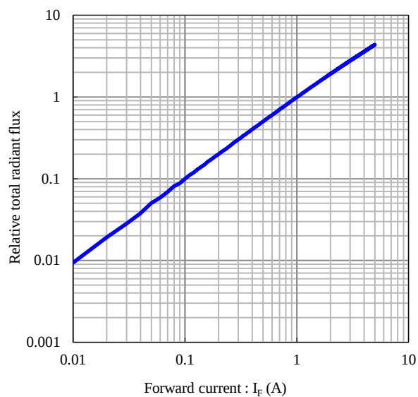
Forward current vs. Relative total radiant flux
