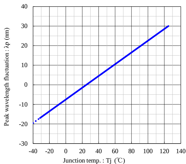
Junction temp. vs. Peak wavelength fluctuation
