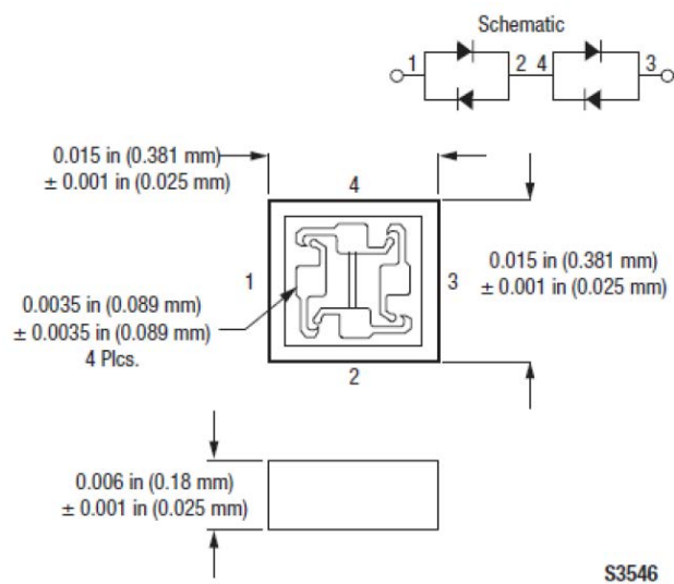
Figure 4. 551-056 Package Dimensions
