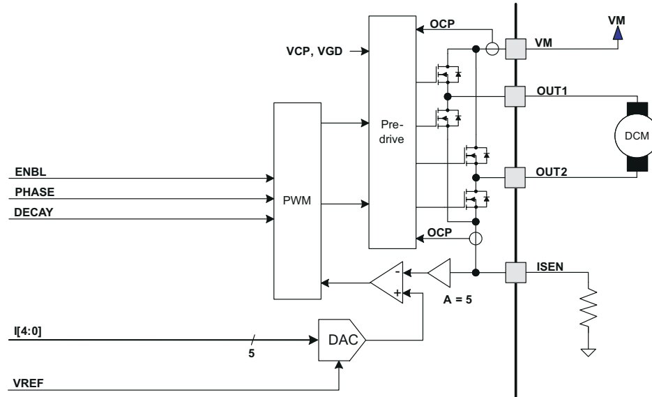
Figure 7-1. Motor Control Circuitry
