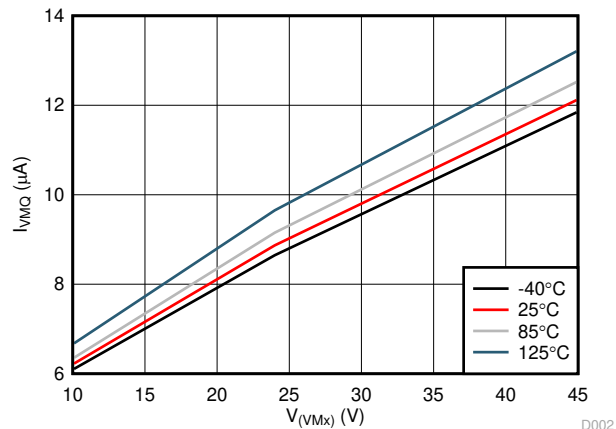
Figure 6-2. I_{VMxQ} vs V_{VMx}
