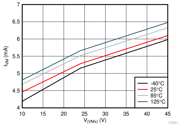
Figure 6-1. I_{VMx} vs V_{VMx}
