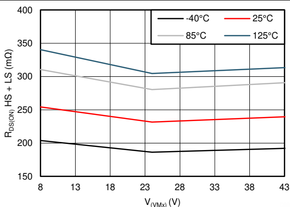
Figure 6-3. R_{DS(ON)} vs V_{VMx}
